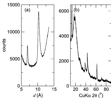
Figure 3. XRD patterns of the nanoscrolls showing (a) the symmetrical Lorentzian reflections at large d -spacings, which is consistent with 003 and 002 reflections (for c \approx 20 Å), and (b) the higher-angle reflections beyond 20^\circ 2\theta , which display the sawtooth profiles associated with hk0 correlations that are typical of a lamellar system with poor registry between layers. Note the large hump near 2\theta \approx 20^\circ , which suggests the presence of amorphous components.
