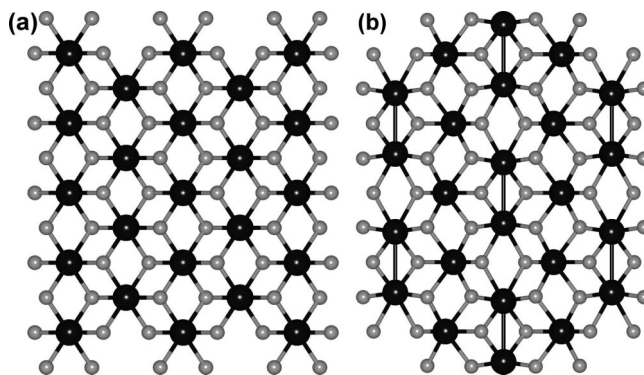
Figure 1. Structure of (a) the high-temperature tetragonal rutile form of \text{VO}_2 and (b) the low-temperature monoclinic form, showing alternating short (indicated by bonds) and long V–V distances. The large dark spheres are vanadium atoms and the small lighter spheres are oxygen atoms.
