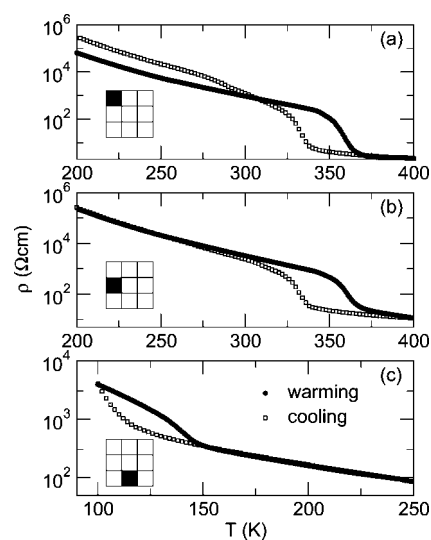
Figure 10. Resistivity as a function of temperature acquired upon warming and cooling, for reduced samples prepared at (a) VO_2 , 400 ^\circ\text{C} , 1 h; (b) VO_2 , 500 ^\circ\text{C} , 1 h; and (c) V_2O_3 , 600 ^\circ\text{C} , 3 h.
